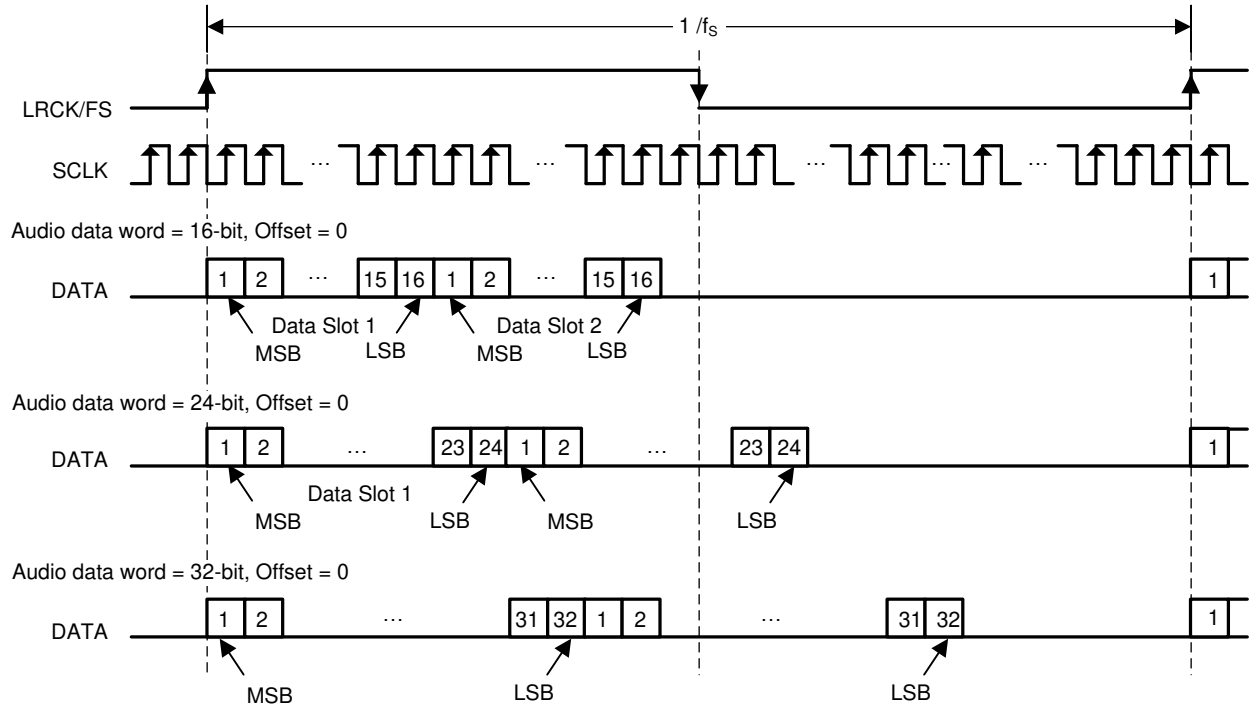
TDM Data Format with OFFSET = 0 In TDM Modes, Duty Cycle of LRCK/FS should be 1x SCLK at minimum. Rising edge is considered frame start.
