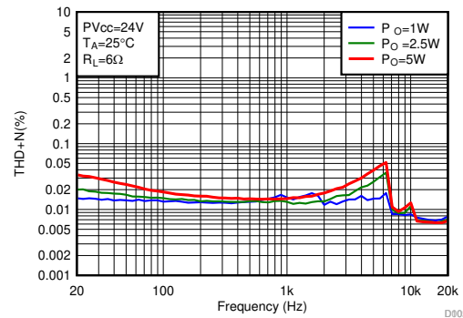
Figure 6-6. THD+N vs Frequency-BTL
