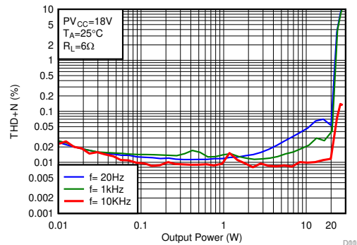
Figure 6-18. THD+N vs Output Power-BTL
