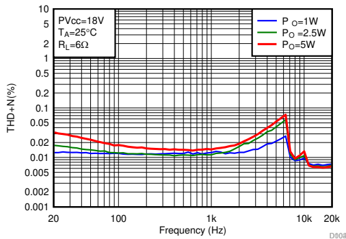
Figure 6-5. THD+N vs Frequency-BTL
