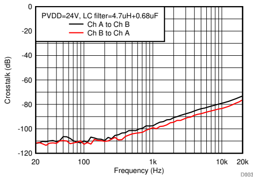
Figure 6-29. Crosstalk
